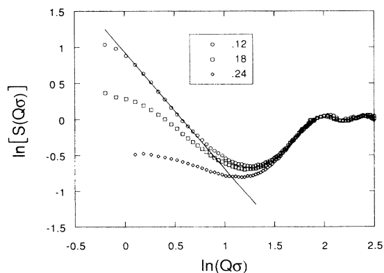
FIG. 2. Structure factors S(Q) for three unsheared gels. Note the signature of a long range correlation at low Q\sigma , with an apparent fractal dimension at \phi=0.12 of d=1.60 . Note the absence of the typical suspension peak, which would appear between about Q\sigma\approx 4 and 6, depending on the volume fraction.
